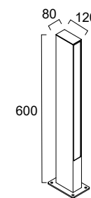
No 4321000 LED 6W • 375Lm 3000K • IP65 • CRI>90 Beam Angle 120°
