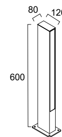
No 4321100 LED 12W • 618Lm 3000K • IP65 • CRI>90 Beam Angle 120°
