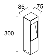
No 4320800 LED 7W • 298Lm 3000K • IP65 • CRI>90 Beam Angle 90°
