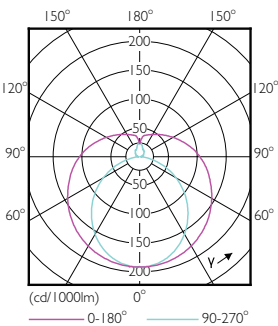
Light Distribution Diagram - Ecofit LEDtube 600mm 8W 865 T8 I RCA
