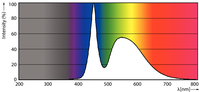
Spectral Power Distribution Colour - Ecofit LEDtube 600mm 8W 865 T8 I RCA
