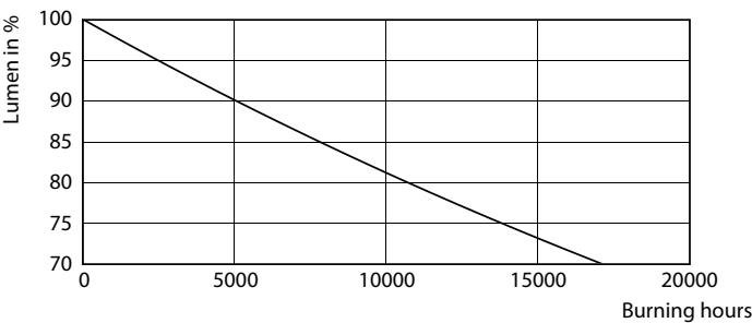
Lumen Maintenance Diagram - Ecofit LEDtube 600mm 8W 865 T8 I RCA
