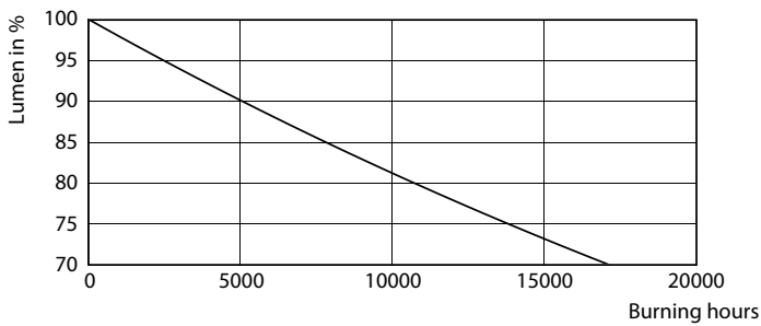
Lumen Maintenance Diagram - Ecofit LEDtube 600mm 8W 840 T8 I RCA
