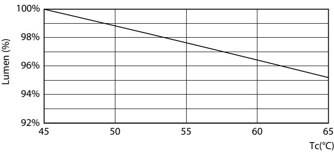
Lumen Maintenance Diagram - Ecofit LEDtube 1200mm 16W 865 T8 I RCA
