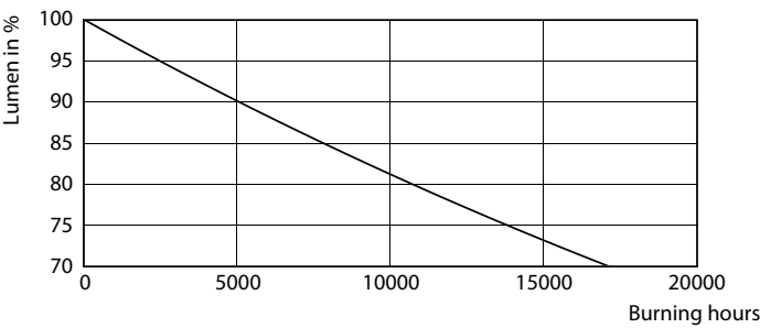
Lumen Maintenance Diagram - Ecofit LEDtube 1200mm 16W 865 T8 I RCA
