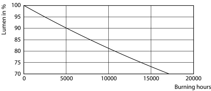
Lumen Maintenance Diagram - Ecofit LEDtube 1200mm 16W 840 T8 I RCA
