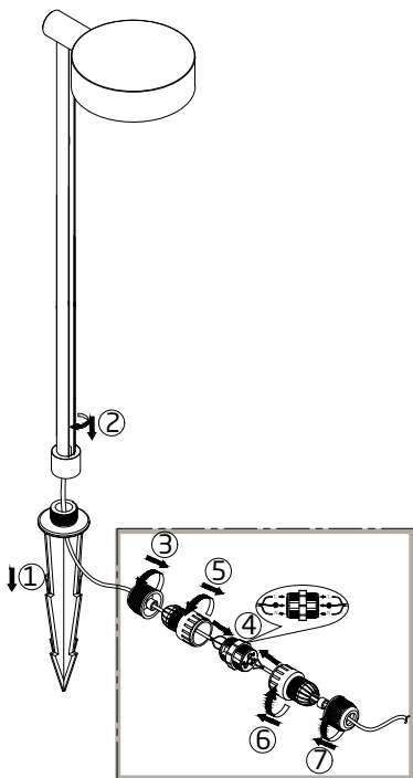
spike mounting
