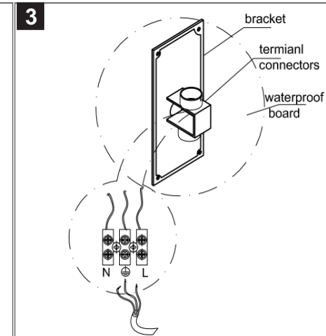
wiring diagram
